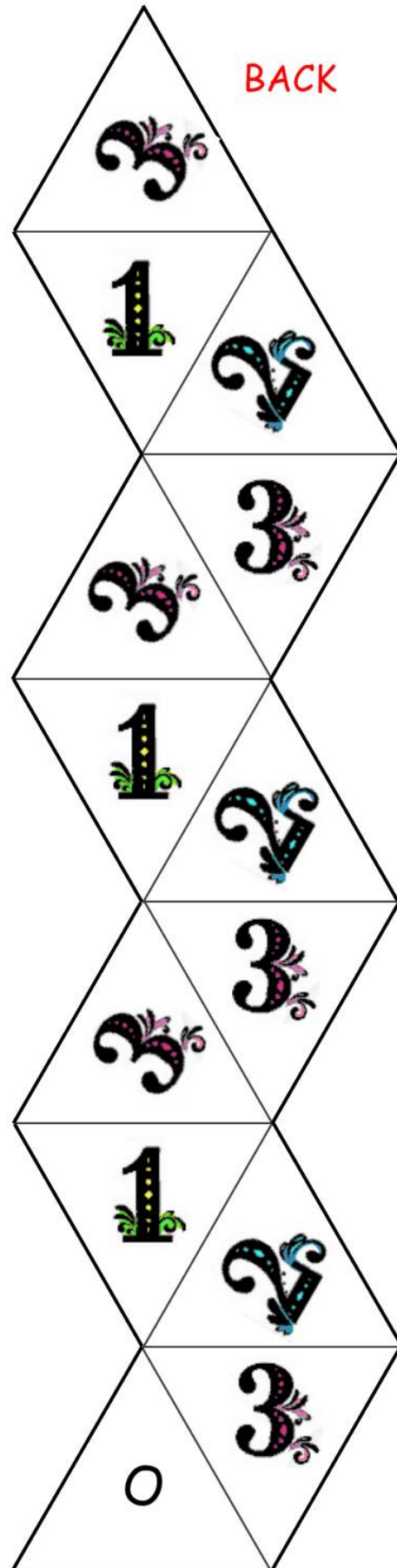
The 1234 Tetraflexagon
